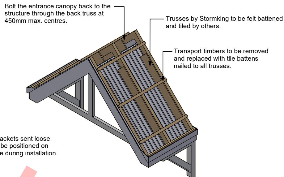
Auxiliary View ( 1 : 25 )
