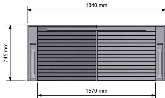
Reflected Plan Elevation ( 1 : 25 )
