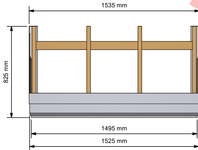
Front View ( 1:20 )
