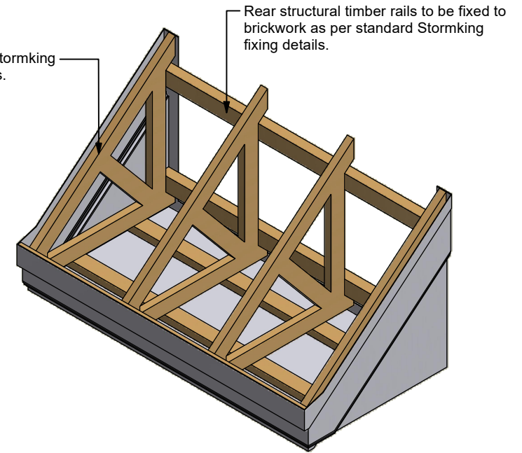
Auxiliary View ( 1:20 )
