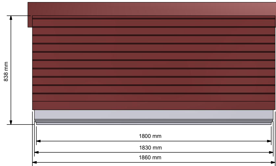
Front Elevation ( 1:15 )
