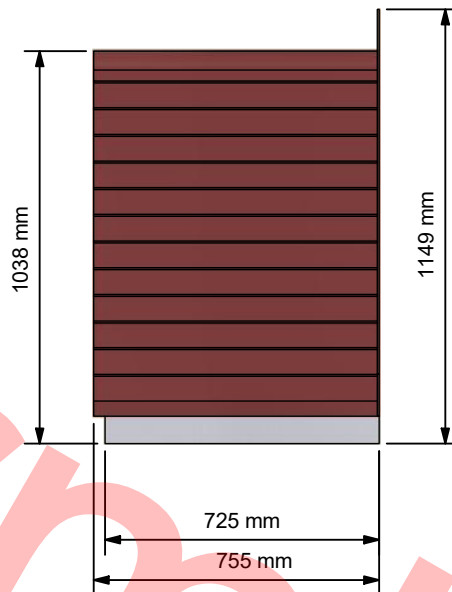
Side View ( 1:20 )
