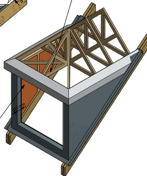
Auxiliary View ( 1:35 )
