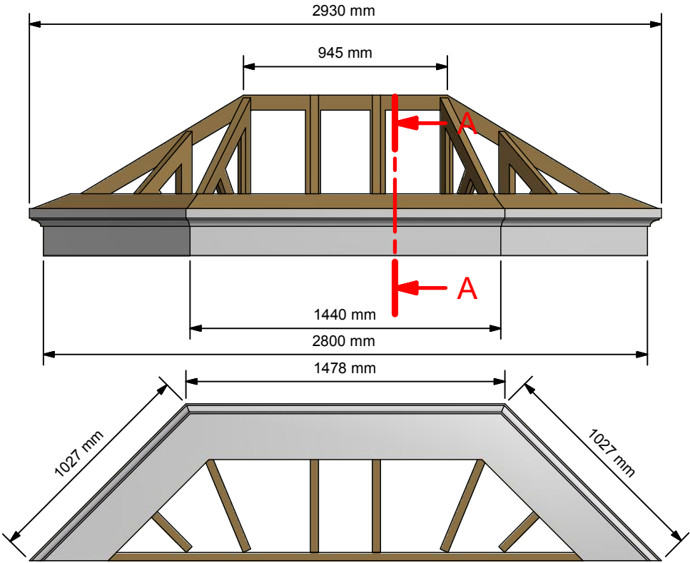
Reflected Plan Elevation ( 1 : 25 )
