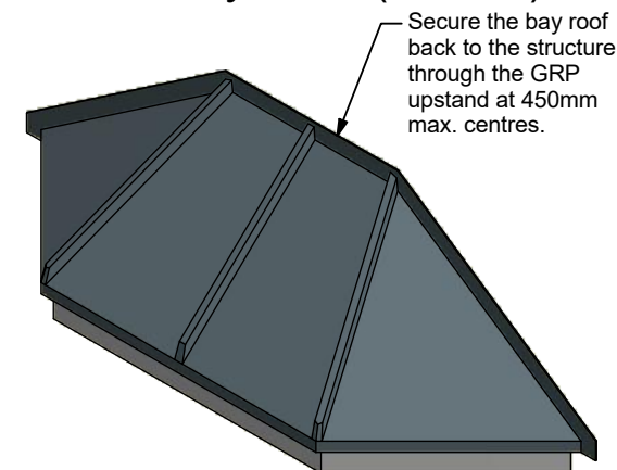
Auxiliary View ( 1 : 30 )
