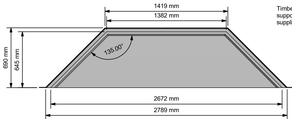
Reflected Plan Elevation ( 1 : 25 )
