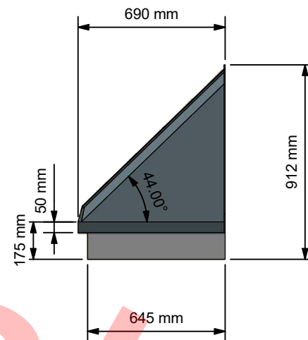
Side Elevation ( 1 : 25 )
