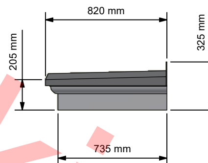
Side Elevation ( 1:25 )
