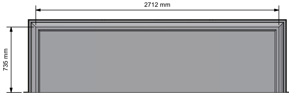
View On Underside ( 1 : 25 )
