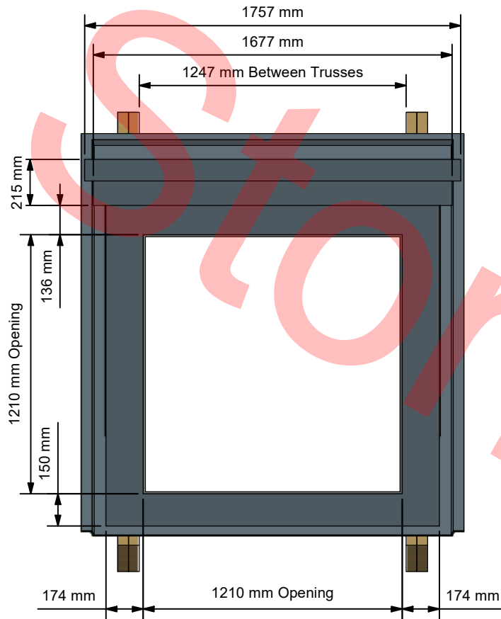
Front Elevation ( 1 : 25 )
