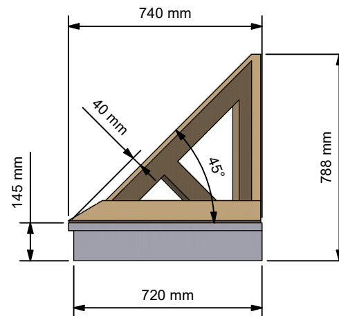
Side Elevation ( 1:20 )
