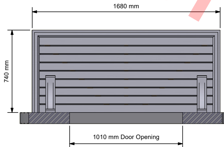
View On Underside Showing Brickwork Dim's. ( 1:20 )
