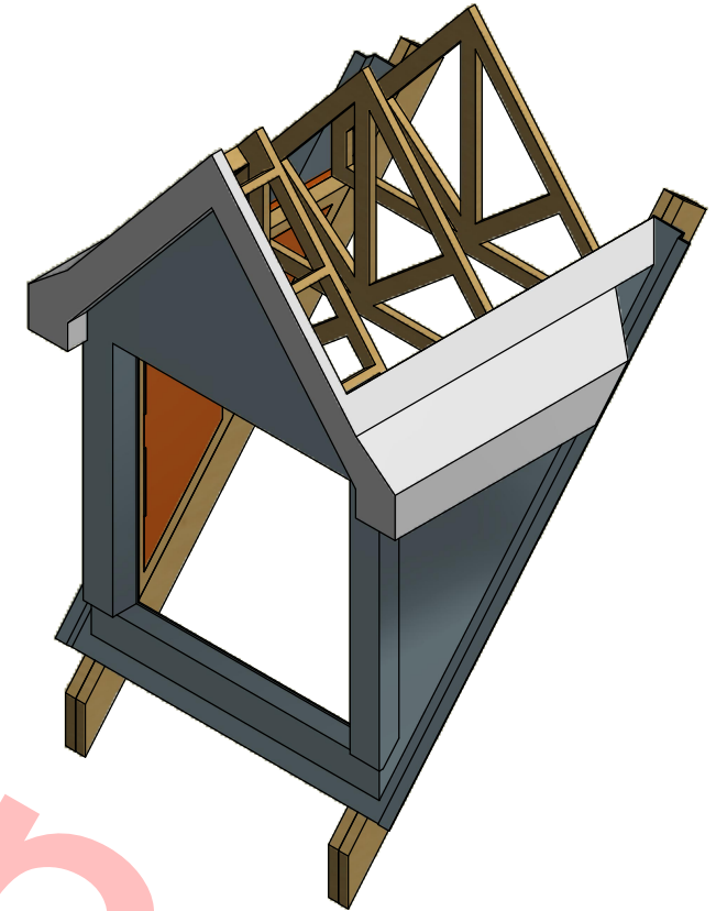
Auxiliary View ( 1 : 30 )
