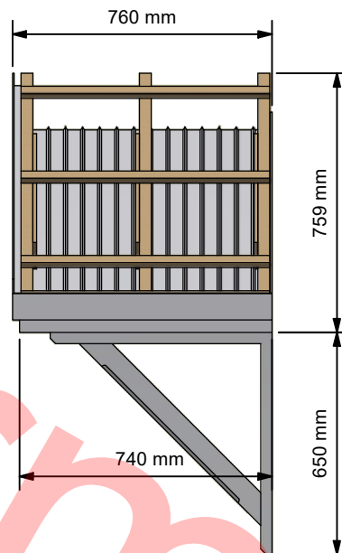
Side Elevation ( 1:20 )
