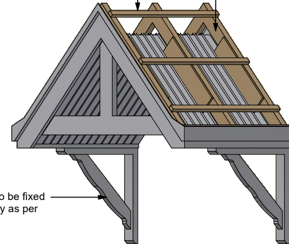
Auxiliary View ( 1:20 )
