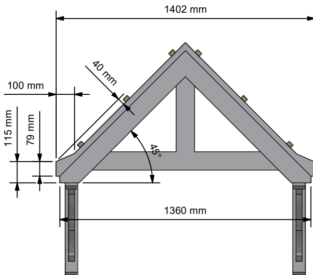
Front Elevation ( 1:20 )
