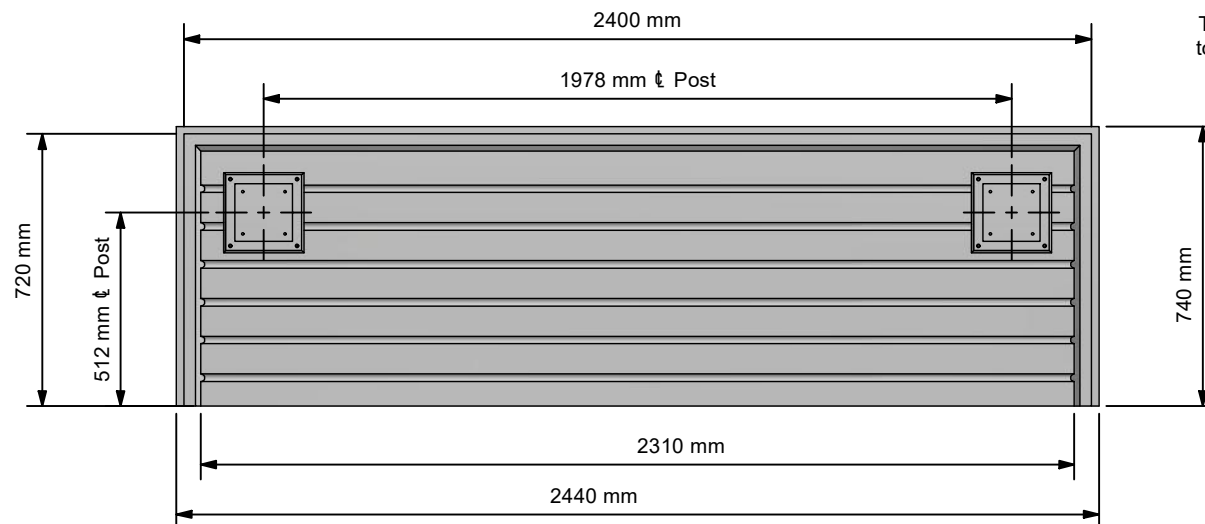
Reflected Plan View ( 1 : 20 )
