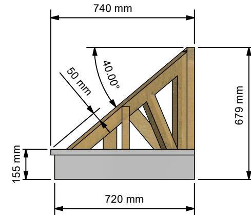
Side Elevation ( 1 : 20 )
