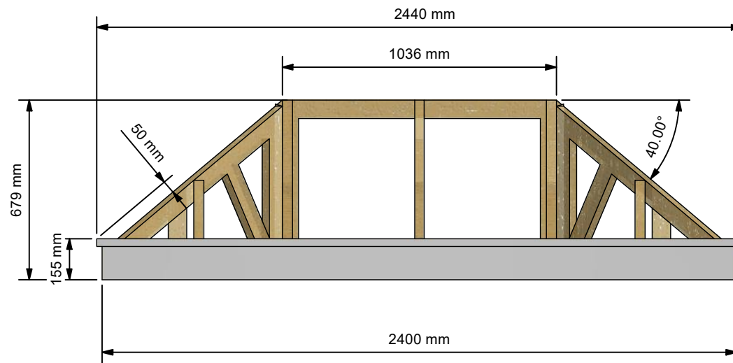
Front Elevation ( 1 : 20 )
