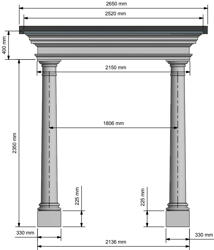
Front Elevation ( 1 : 25 )
