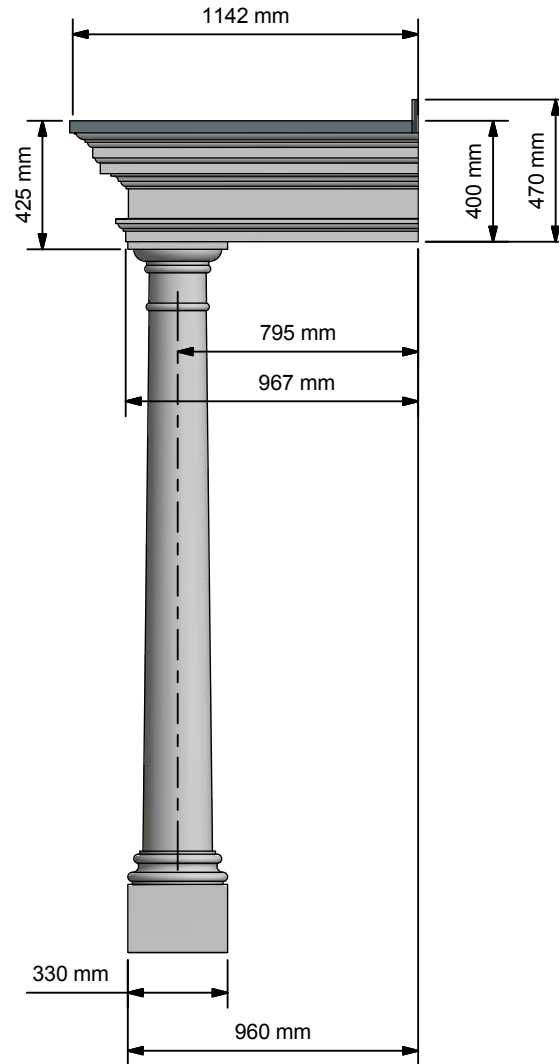
Side Elevation ( 1 : 25 )
