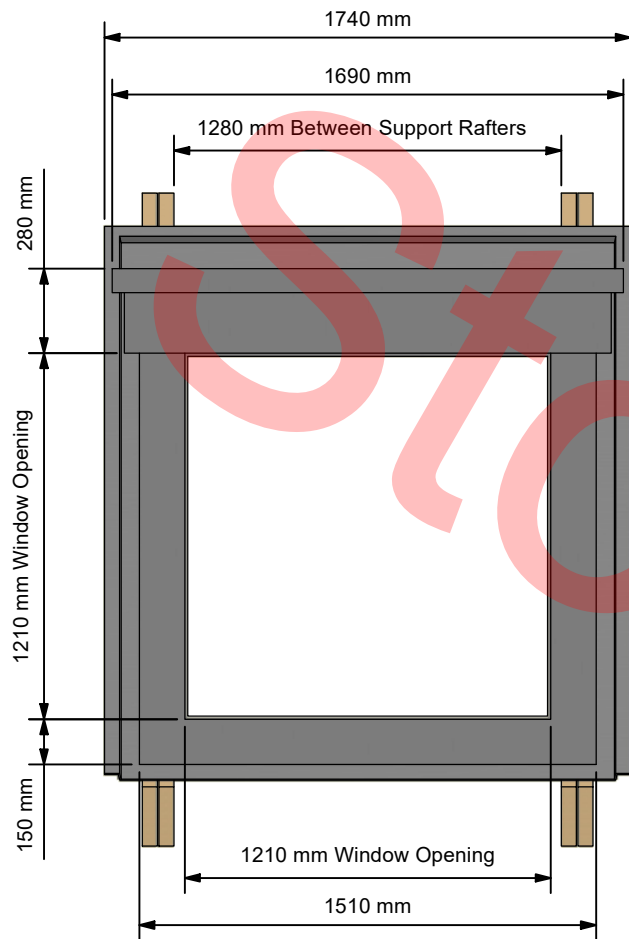
Front Elevation ( 1:25 )
