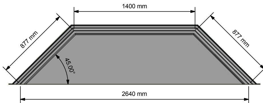
Reflected Plan View ( 1:25 )
