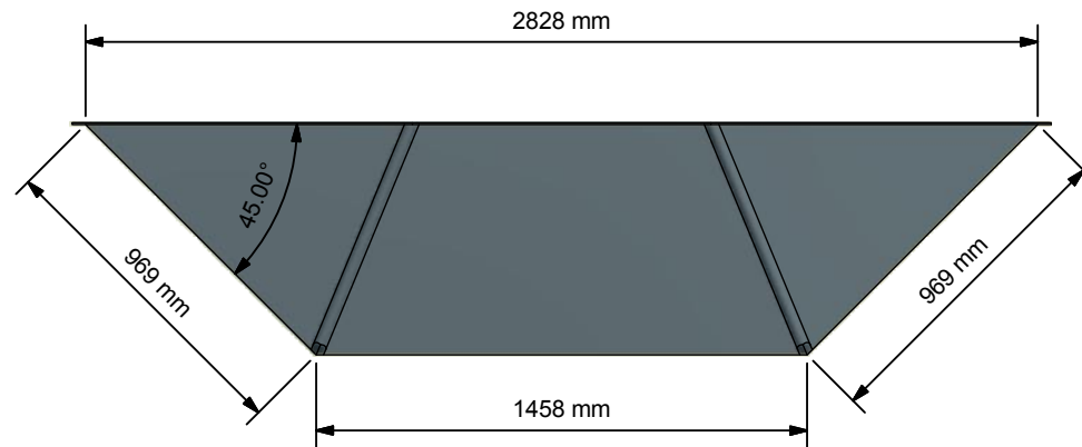
Plan View ( 1:25 )
