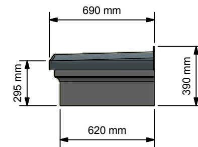
Side Elevation ( 1:25 )
