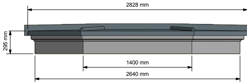
Front Elevation ( 1:25 )
