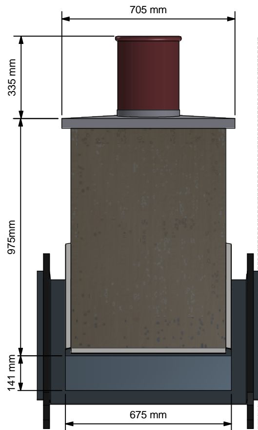
Front Elevation ( 1:15 )
