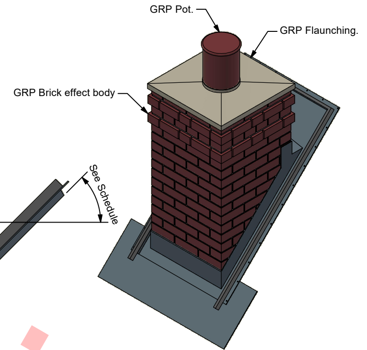
Auxiliary View ( 1 : 25 )
