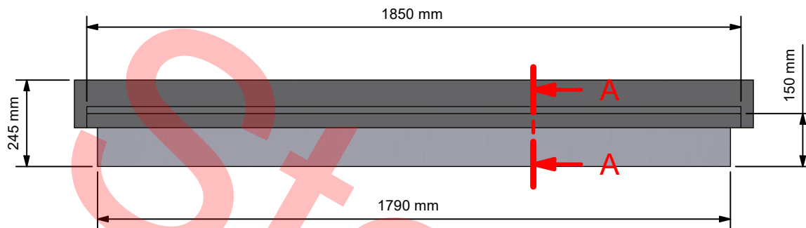
Front Elevation ( 1 : 15 )
