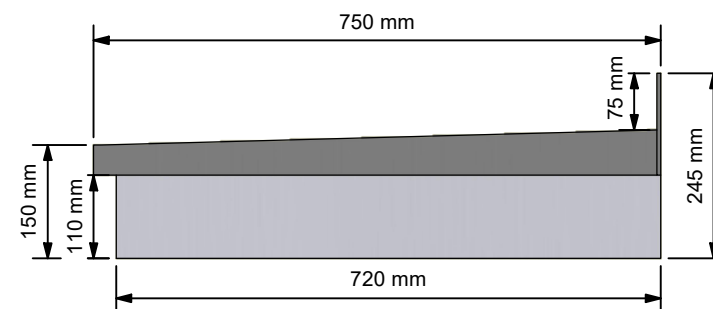
Side Elevation
