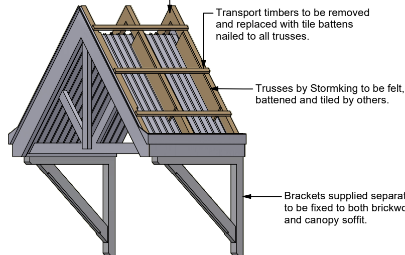
Auxiliary View ( 1 : 25 )
