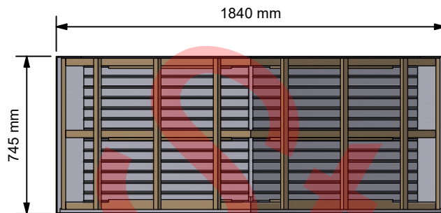
Plan View ( 1:25 )
