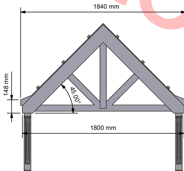
Front Elevation ( 1:25 )
