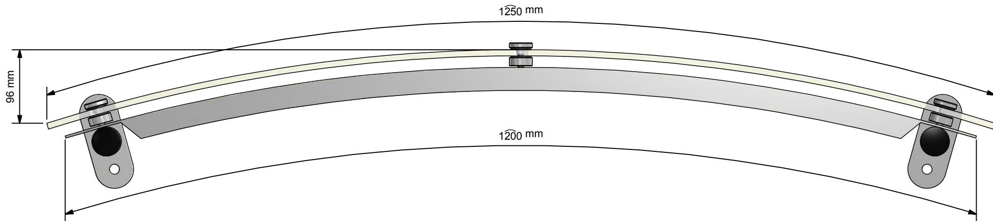
Front Elevation ( 1 : 5 )
