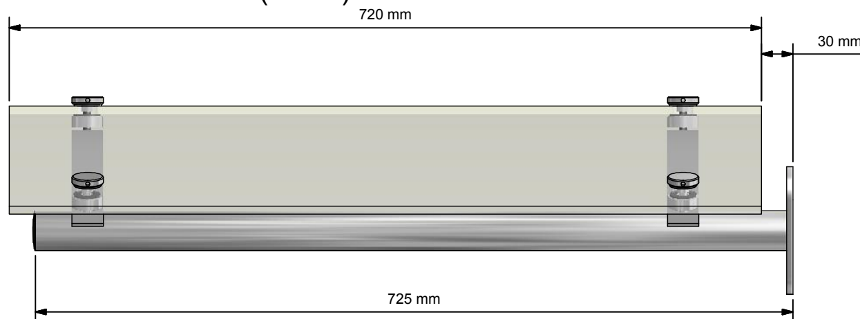
View A ( 1 : 5 )
