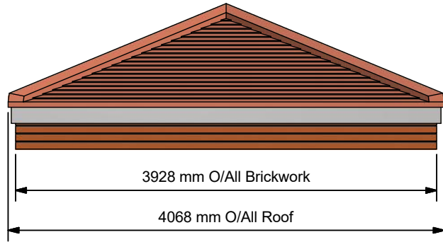
Typical Elevation ( 1:50 )
