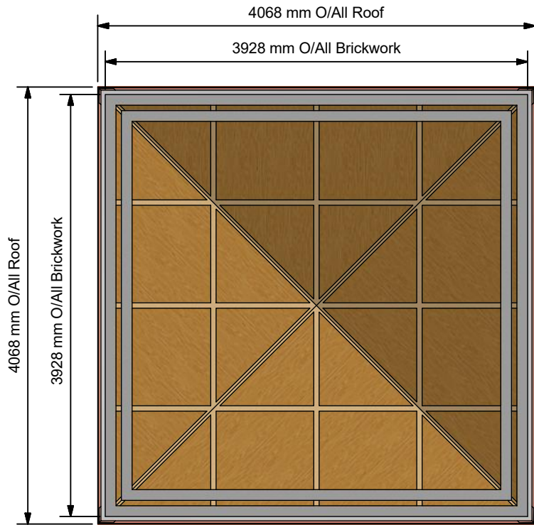
View On Underside Showing Brickwork Dims. ( 1:50 )
