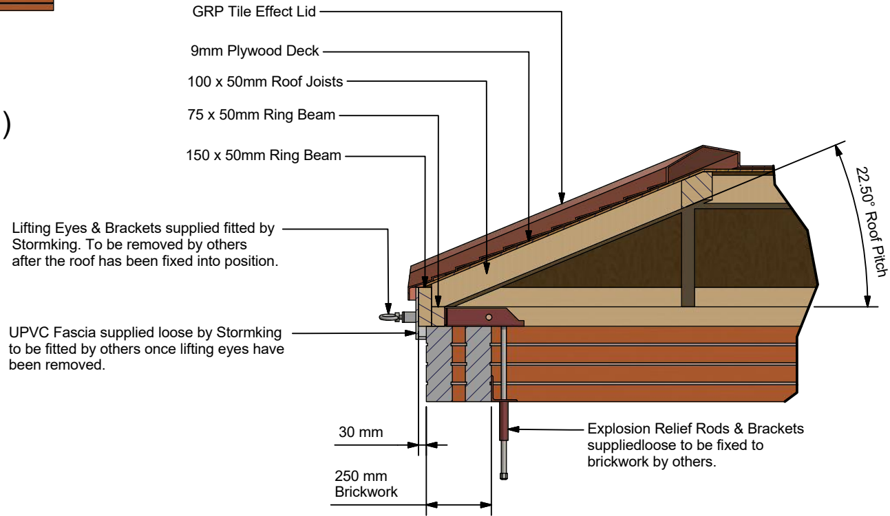
Auxiliary Section A-A ( 1:20 )
