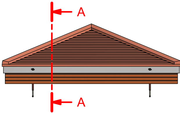
Typical Elevation ( 1:50 )
