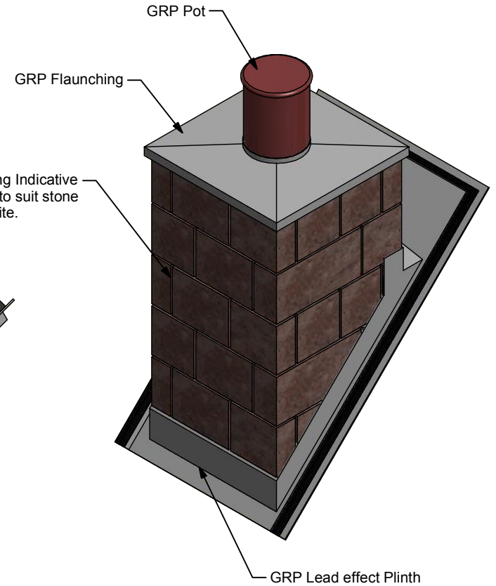
Auxiliary View ( 1 : 20 )
