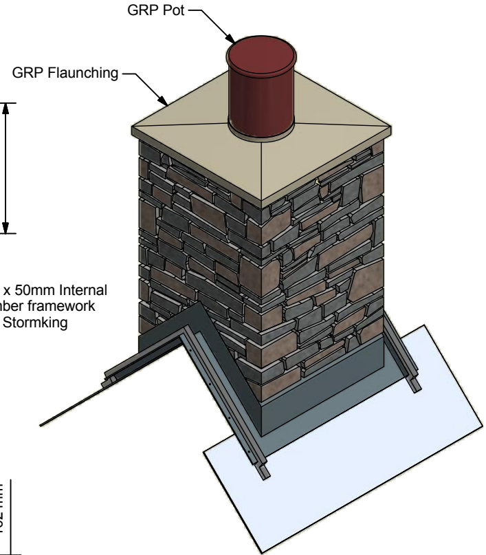
Auxiliary View ( 1:20 )
