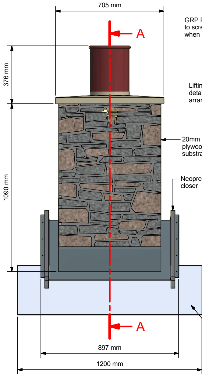
Typical Elevation ( 1:15 )
