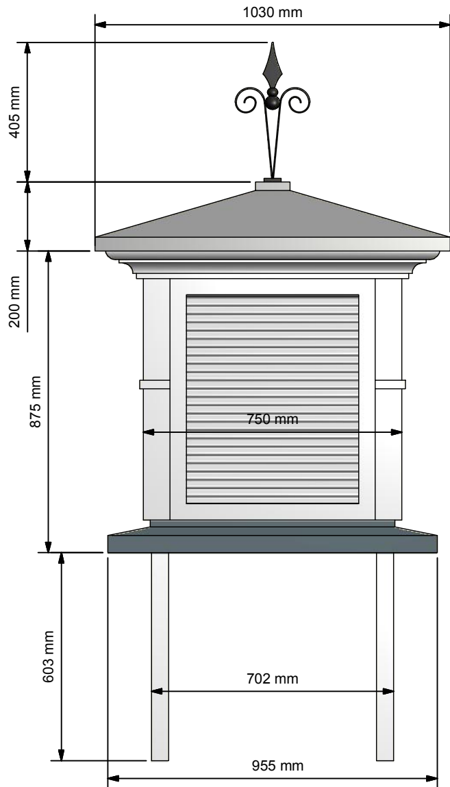
Typical Elevation ( 1 : 15 )
