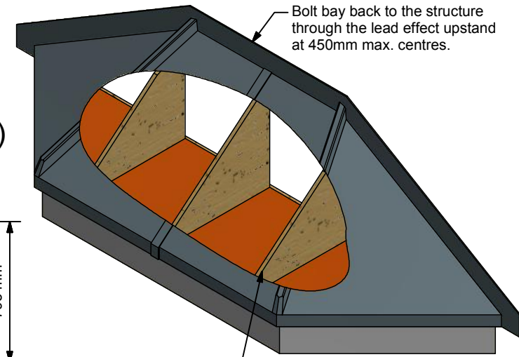
Auxiliary View ( 1 : 20 )
