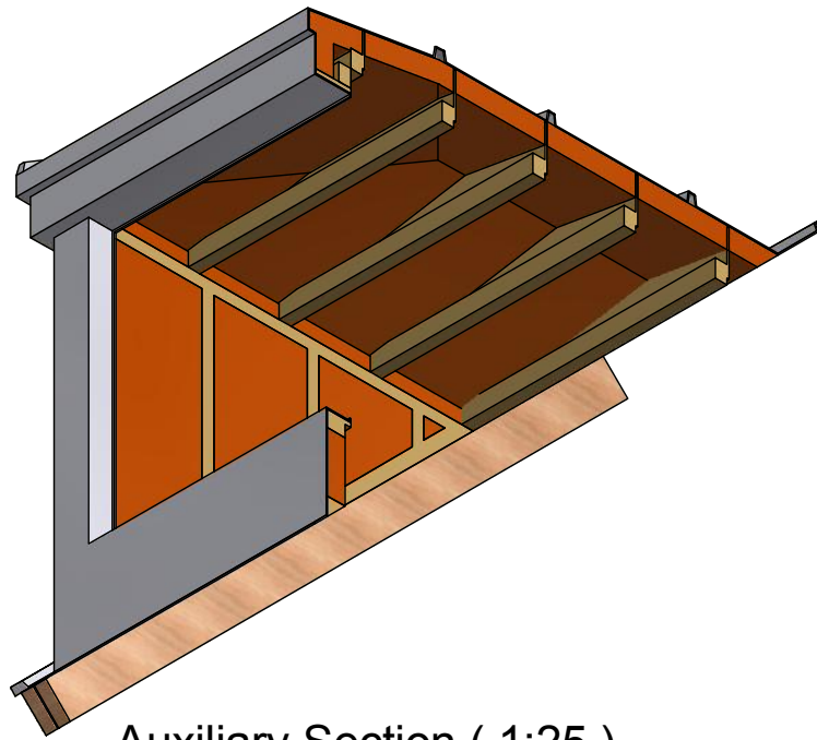
Auxiliary Section ( 1:25 )
