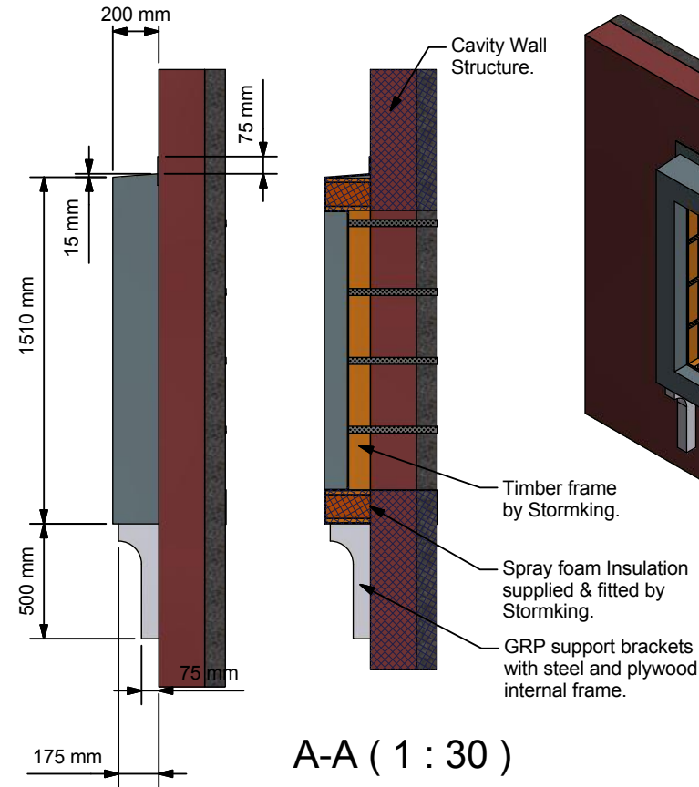
Side Elevation ( 1 : 30 )
