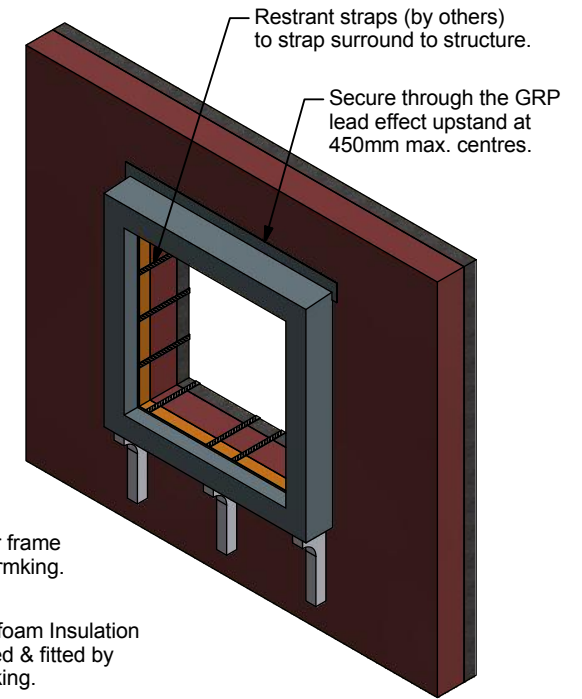
Auxiliary View ( 1 : 40 )
