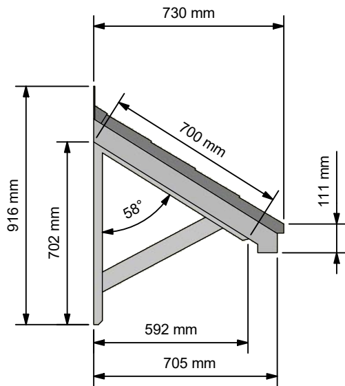
Side Elevation ( 1:20 )
