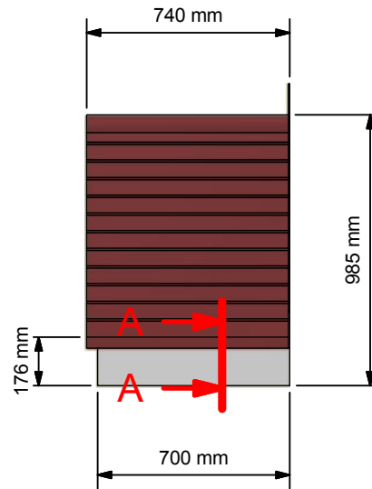
Side Elevation ( 1 : 25 )
