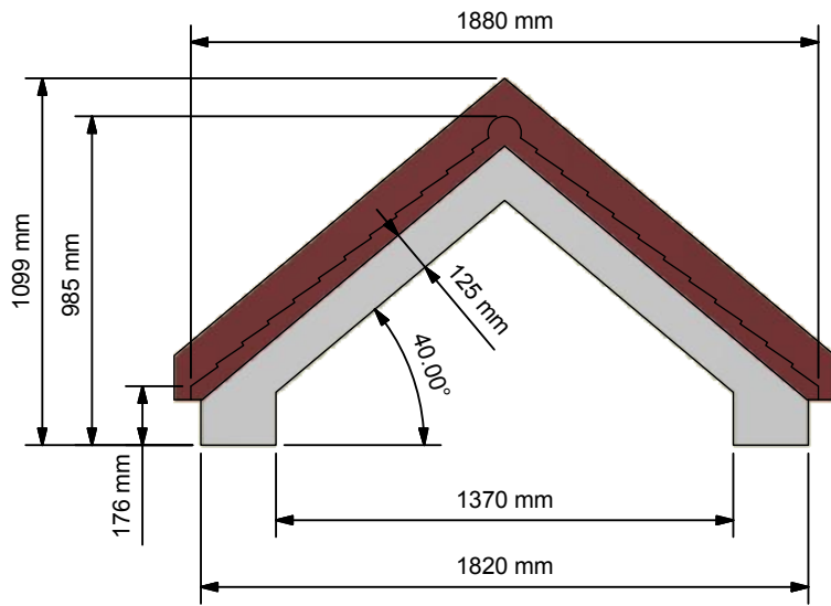
Reflected Plan Elevation ( 1 : 25 )
