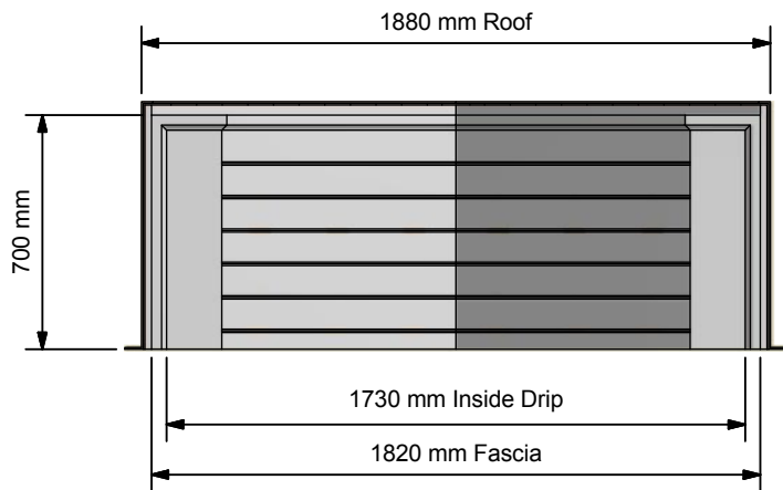
Reflected Plan Elevation ( 1 : 25 )
