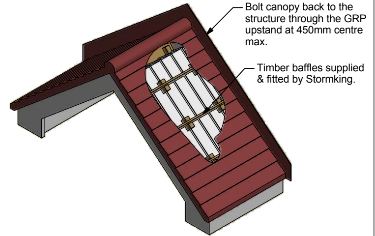
Auxiliary View ( 1 : 25 )
