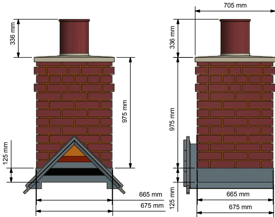
Gable Elevation ( 1:20 )
