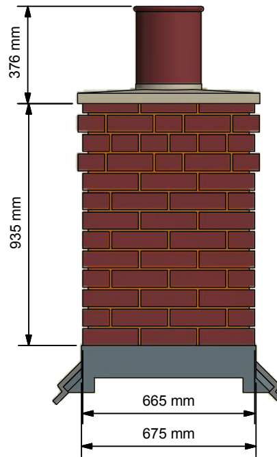
Roof Elevation ( 1:20 )
