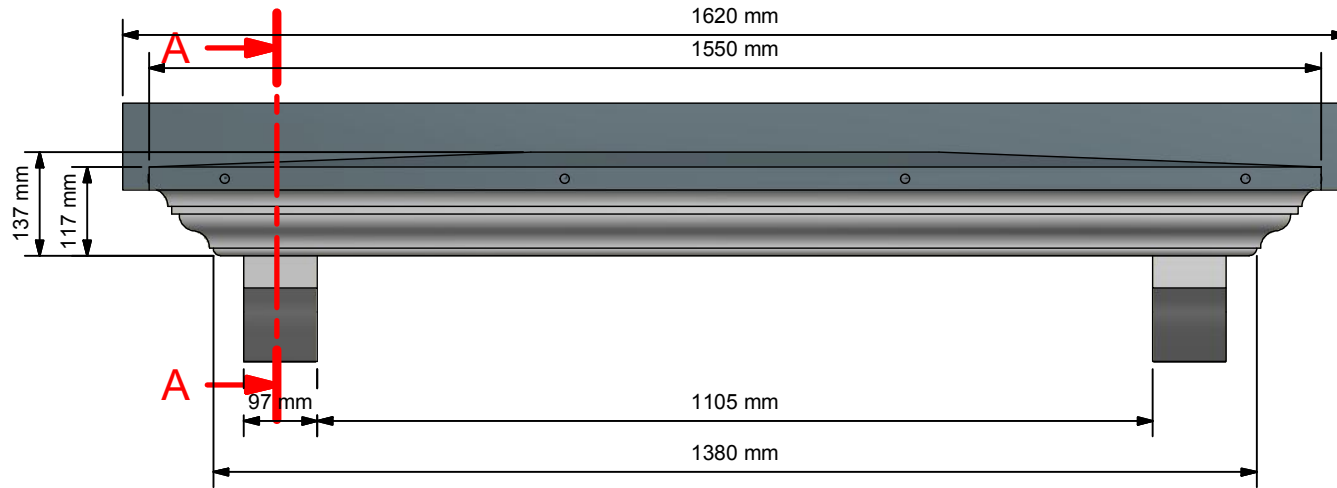
Front View ( 1:10 )
