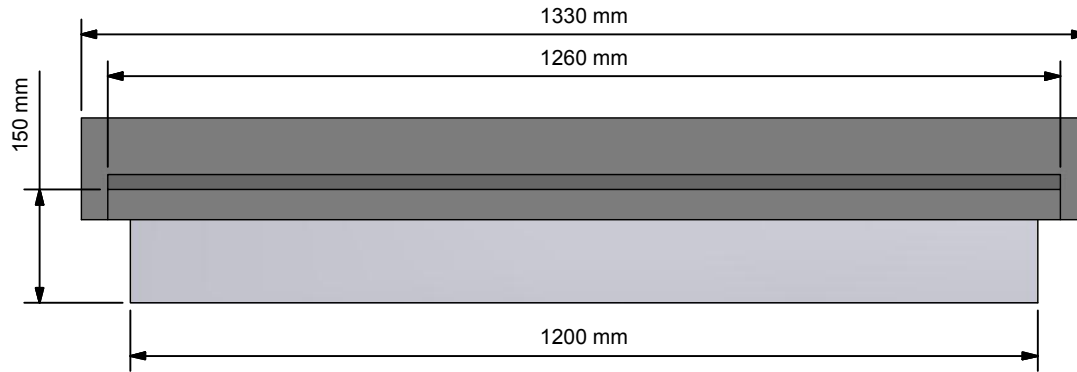
Front Elevation ( 1 : 10 )
