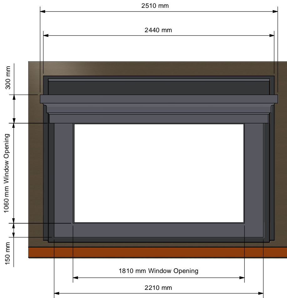
Front Elevation ( 1:25 )
