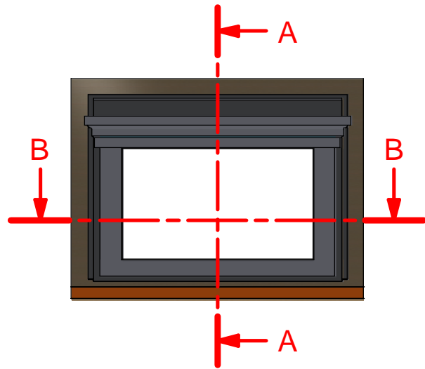
Front Elevation ( 1:50 )
