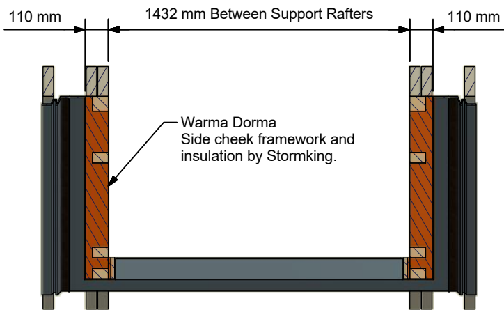
Front Elevation ( 1 : 50 )
