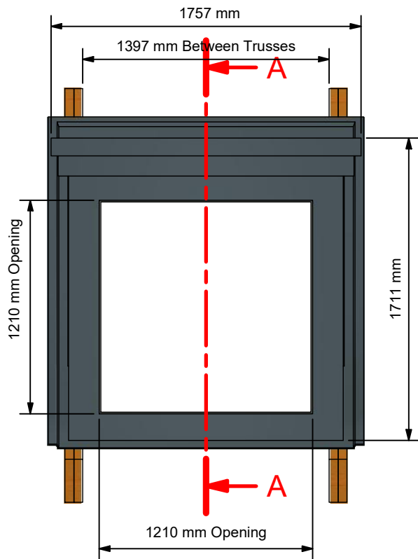
Front Elevation ( 1 : 30 )
