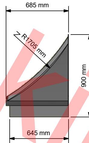
Side Elevation ( 1:25 )
