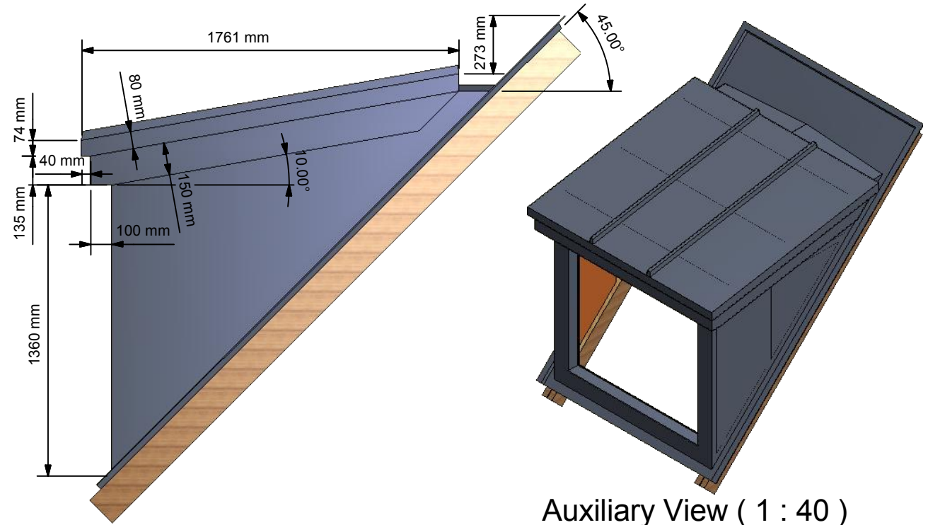
Side Elevation ( 1 : 25 )
