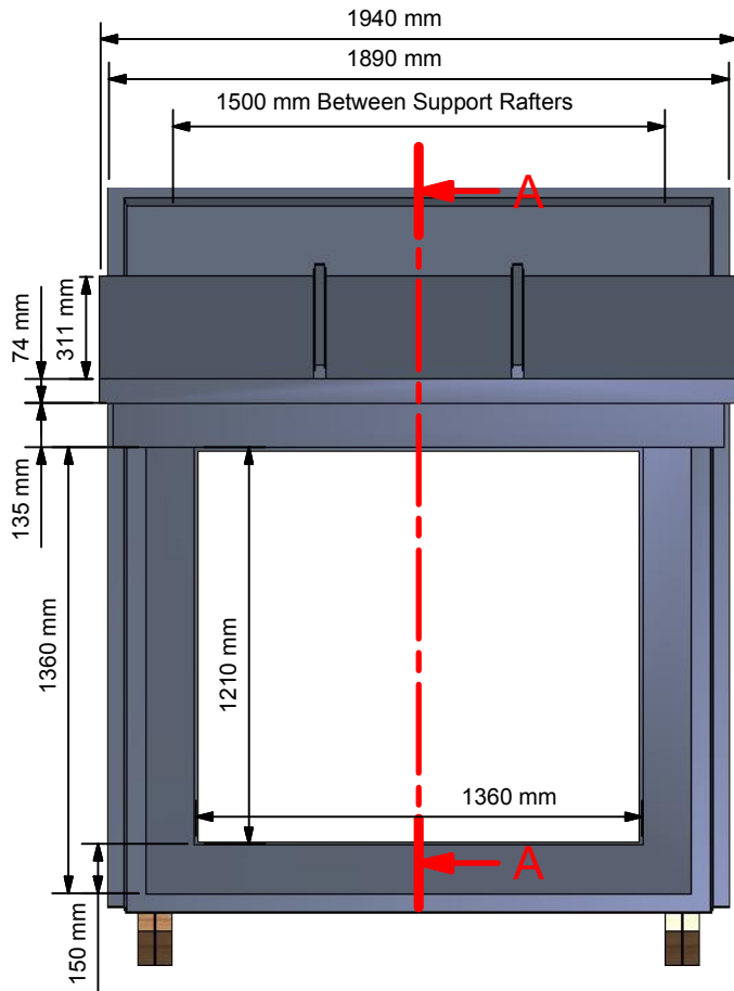
Front Elevation ( 1 : 25 )
