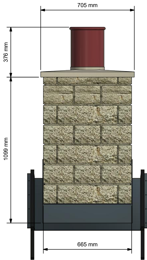
Typical Elevation ( 1:15 )
