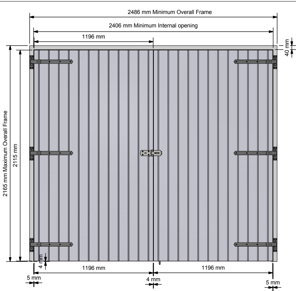
Front Elevation ( 1 : 20 )
