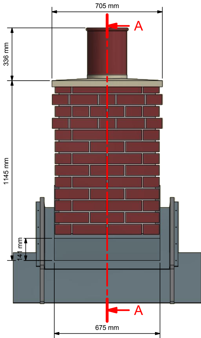
Typical Elevation ( 1:15 )
