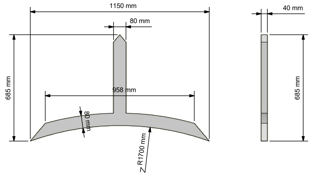
Front Elevation ( 1:15 )
