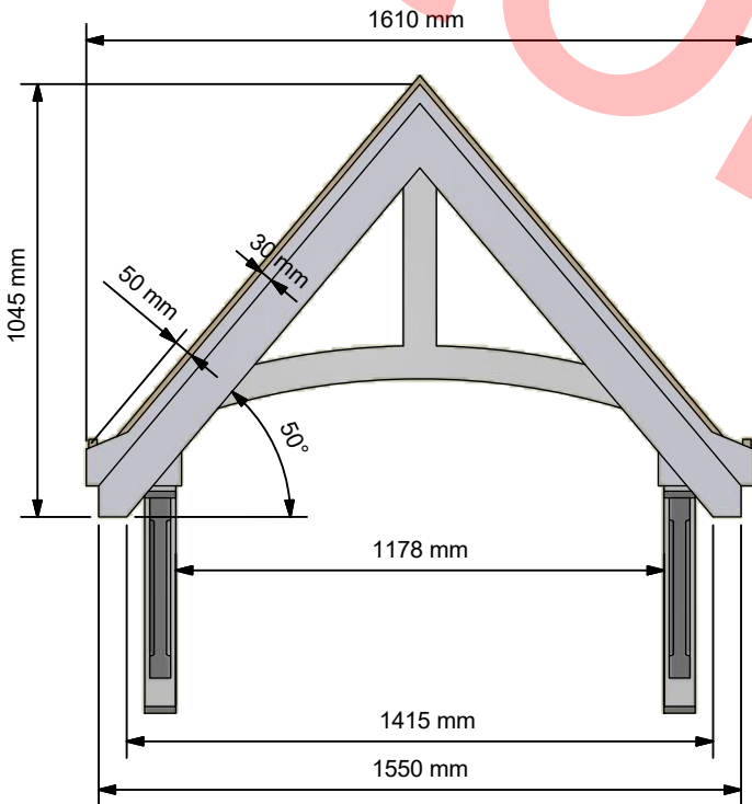
Front Elevation ( 1:20 )
