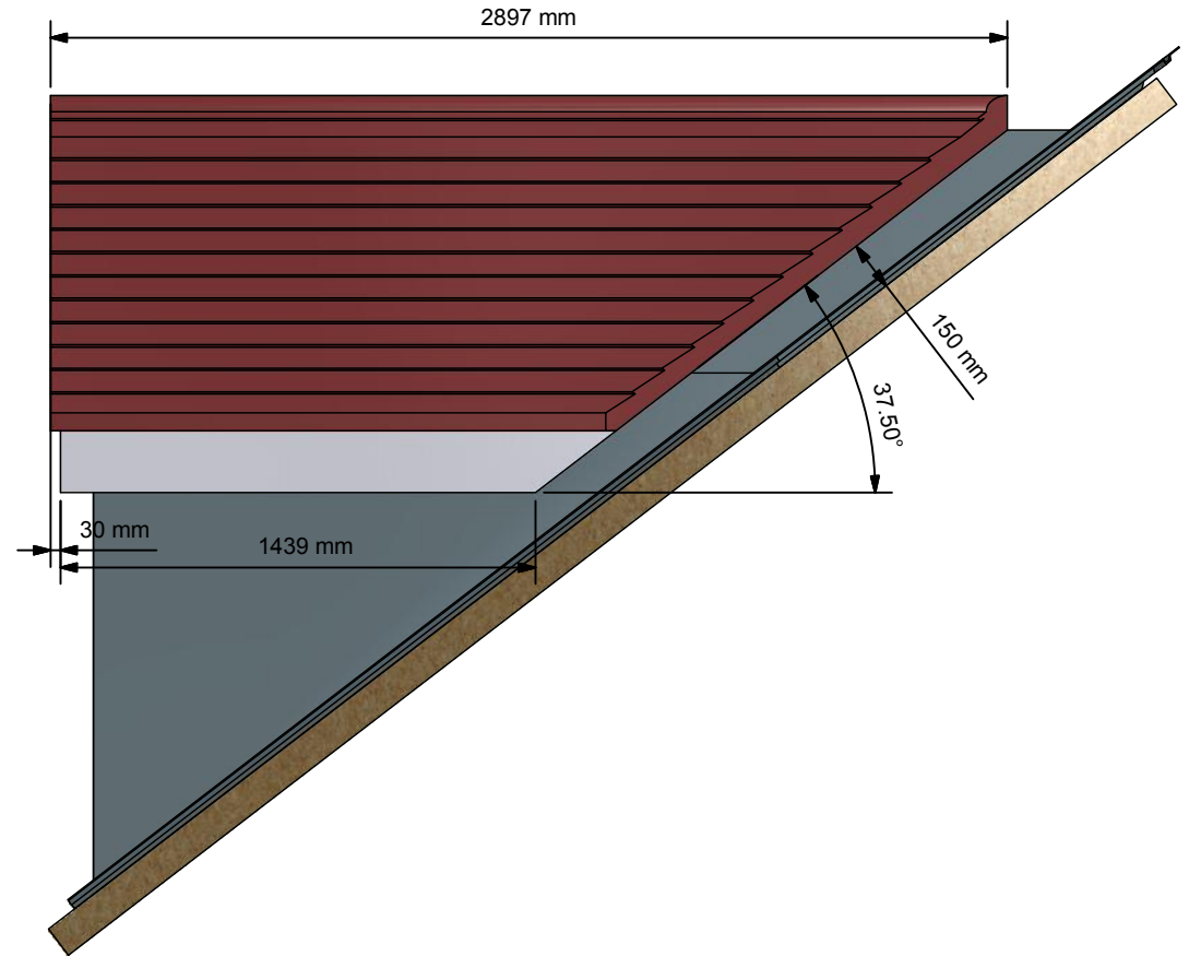
Side Elevation ( 1 : 25 )
