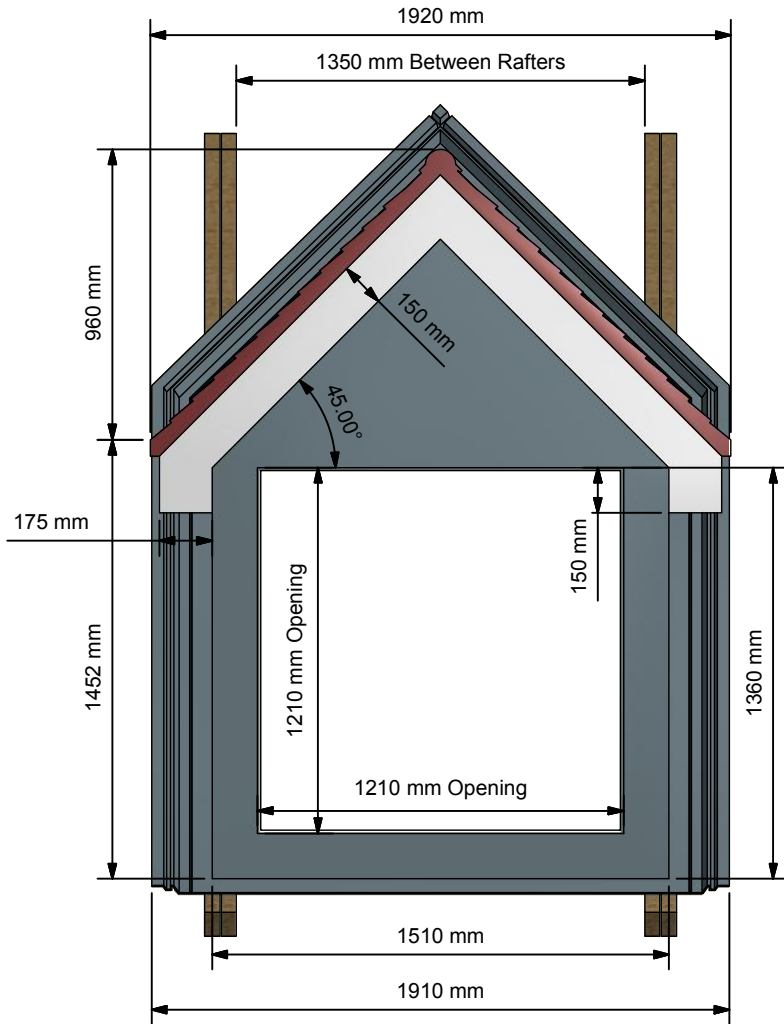
Front Elevation ( 1 : 25 )
