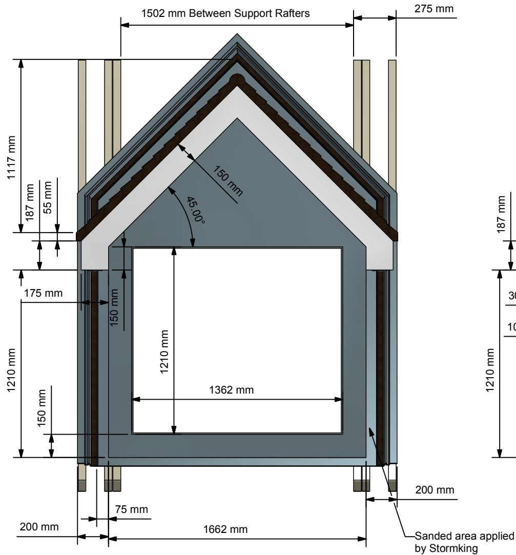
Front Elevation ( 1 : 25 )
