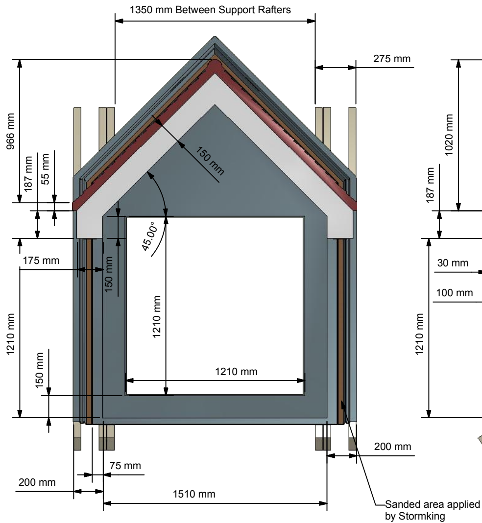
Front Elevation ( 1 : 25 )
