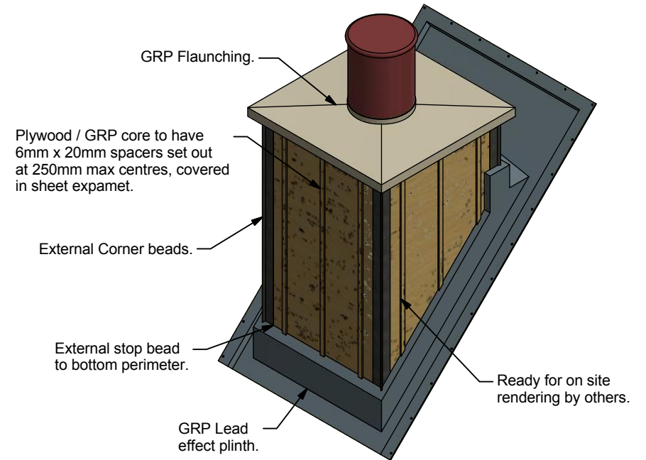
Auxiliary View ( 1:20 )
