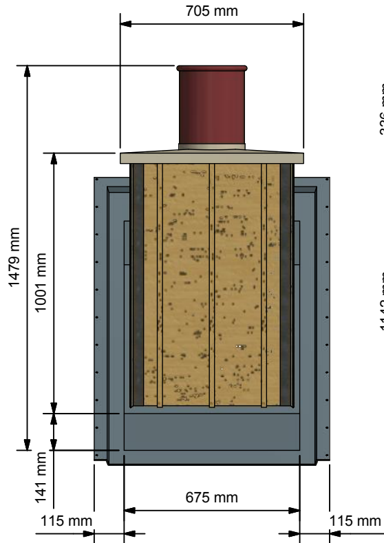
Front Elevation ( 1 : 20 )
