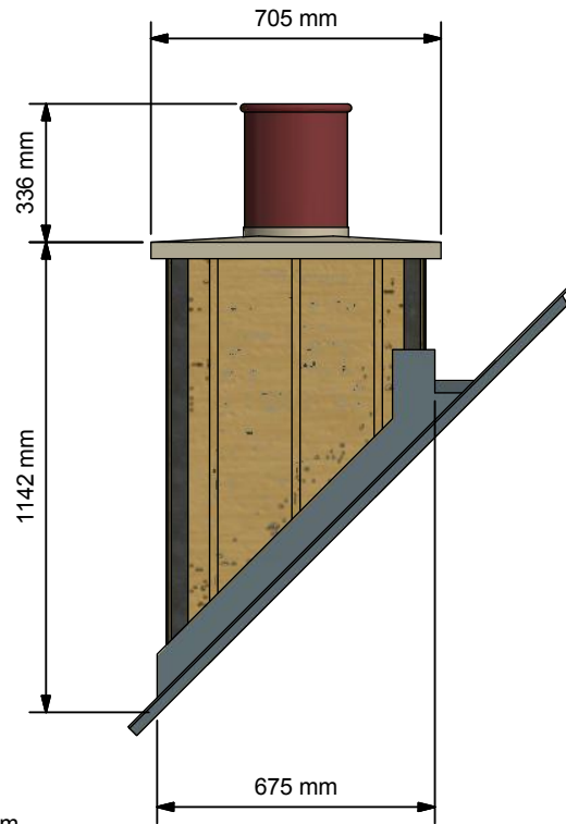
Side Elevation ( 1 : 20 )
