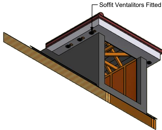
Auxiliary View ( 1:40 )
